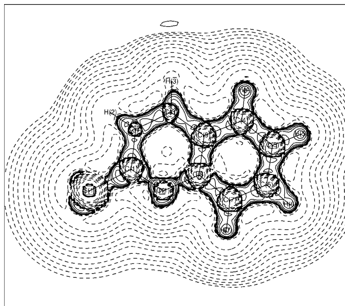
Figure 6 Laplacian [\nabla^2\rho_b(\mathbf{r})] distribution in the plane of the molecule. Contours are drawn at logarithmic intervals in -\nabla^2\rho_b e \text{\AA}^{-5} . The solid lines are positive contours and the broken lines are negative contours.
