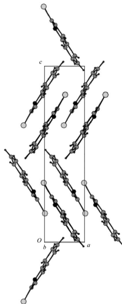
Figure 2 Molecular packing of the crystal viewed along the b axis.
