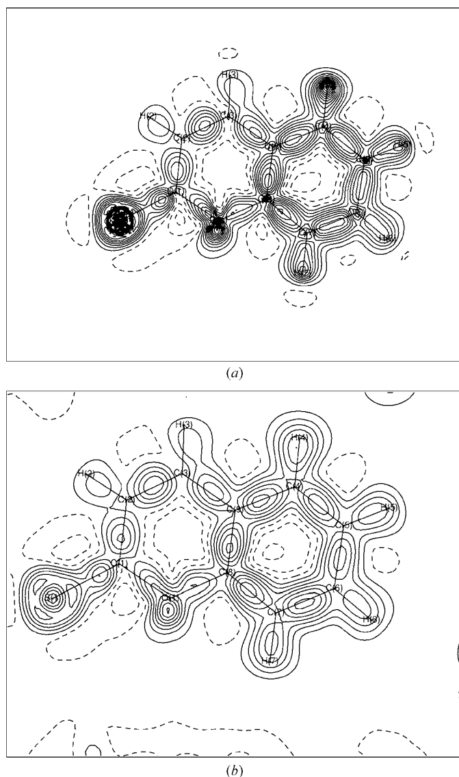
Figure 4 (a) Dynamic-deformation density map in the plane of the molecule. The first positive contour is at 0.05 \text{ e } \text{Å}^{-3} and the contour levels are at 0.1 \text{ e } \text{Å}^{-3} intervals. The first negative contour is at -0.05 \text{ e } \text{Å}^{-3} and the contour levels are at -0.1 \text{ e } \text{Å}^{-3} intervals. The solid lines are positive contours and the broken lines are negative contours. (b) Static-deformation density map in the plane of the molecule. The positive contour levels are at 0.1 \text{ e } \text{Å}^{-3} intervals and the negative contour levels are at -0.1 \text{ e } \text{Å}^{-3} intervals. The solid lines are positive contours and the broken lines are negative contours.
